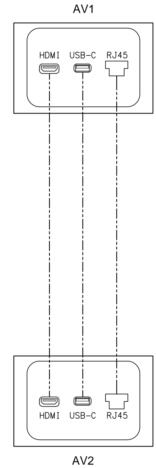
DETAIL TYPICAL AV1 / AV2 FACEPLATES NOT TO SCALE
